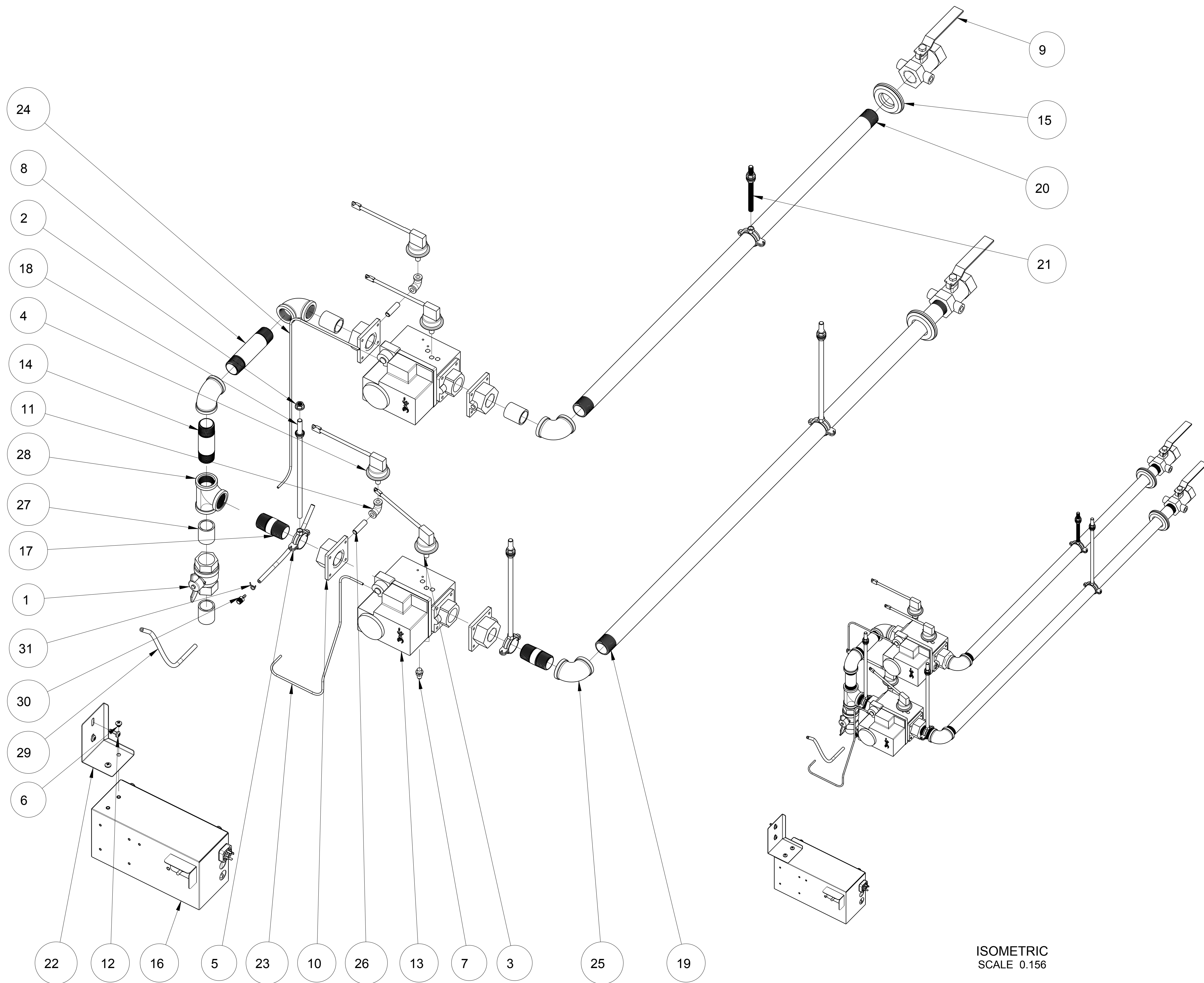
EXPLODED SCALE 0.234
